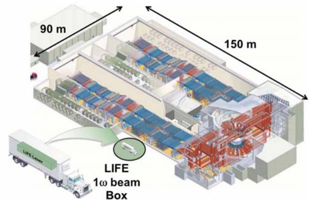
Fig. 2. LIFE beamlines (8.1 kJ, 1\omega , 16 Hz) are configured into a box with dimensions 10.5 \times 2.2 \times 1.35 \text{ m} to allow offsite factory manufacture, truck transportation, and ease of maintenance consistent with power plant operational requirements. This scale is shown in comparison to NIF.
