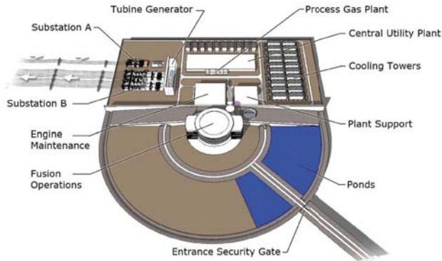
Fig. 1. The LIFE power plant integrates the fusion operations building (100 m diameter) with an engine maintenance area, tritium plant, and conventional utilities on a site consistent in scale with existing baseload plants.
